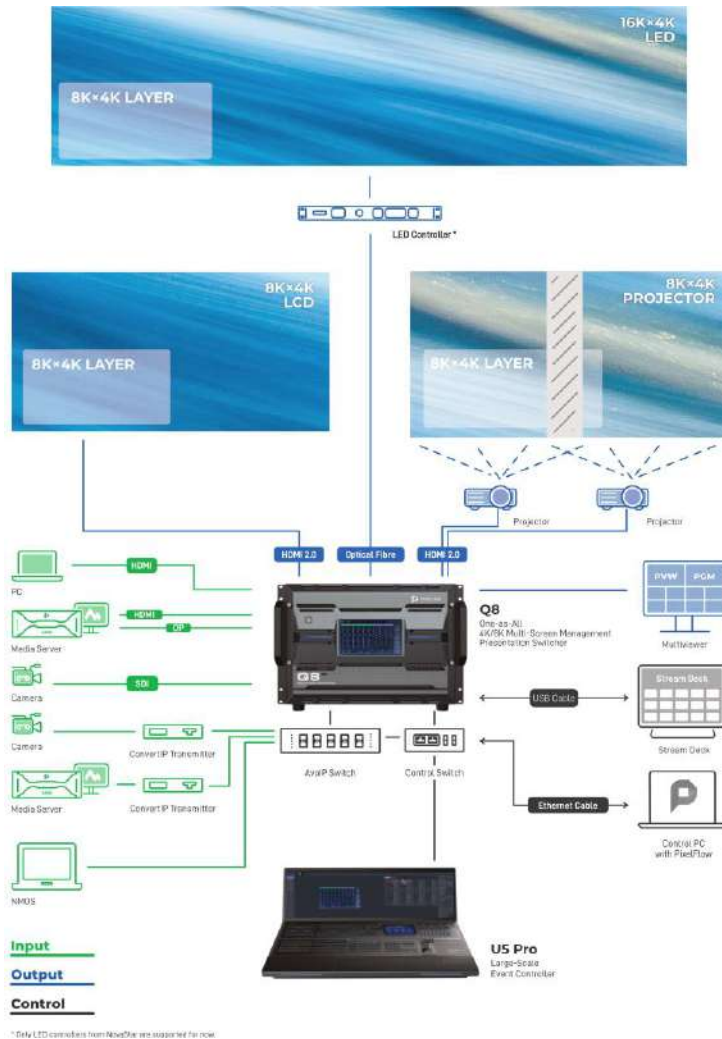
Figure 4-5 Q8+U5/U5 Pro+PixelFlow
