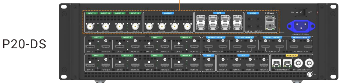
P_12G SDI_DANTE Audio-OPT Combo Card
