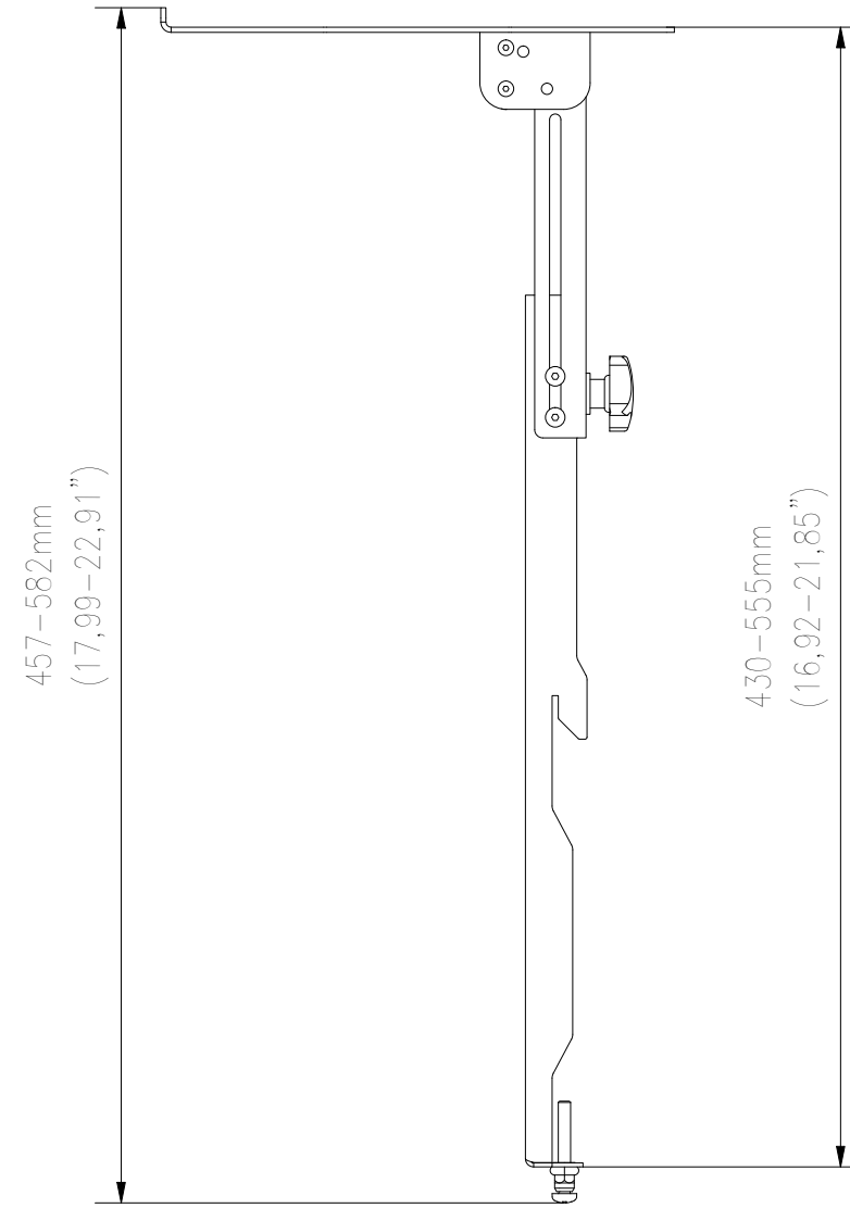
SIDE VIEW
