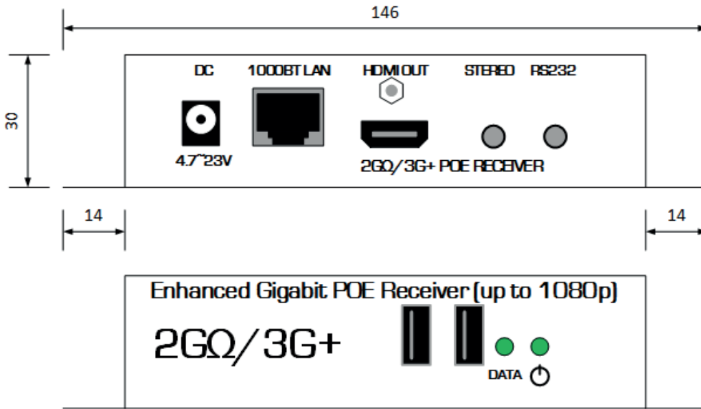
515PoE Front/Back
