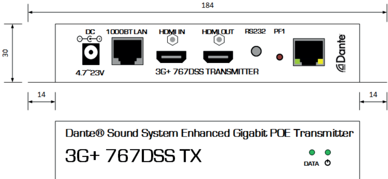
767DSS Front/Back
