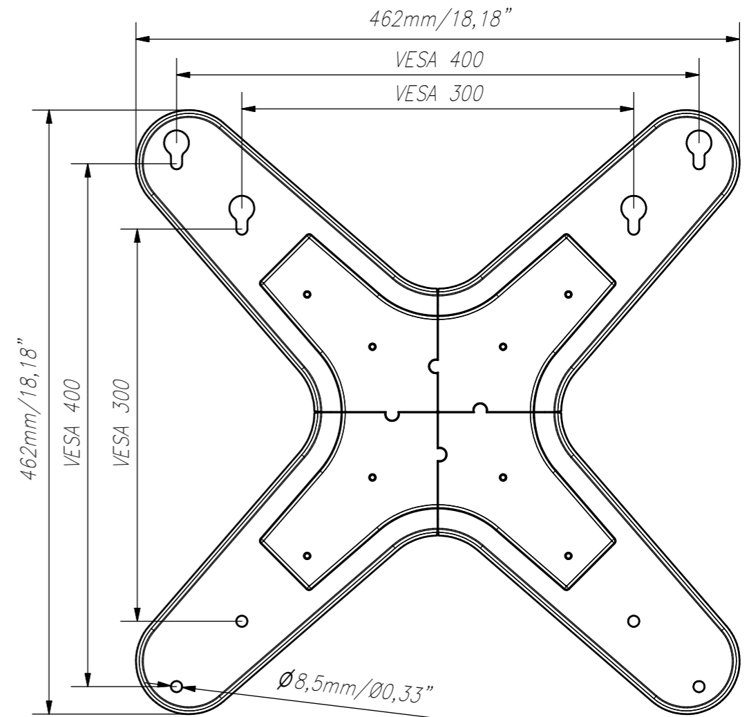
VESA 300-400 adaptery / VESA 300-400 adapters
