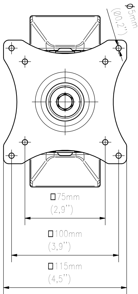
FRONT VIEW
