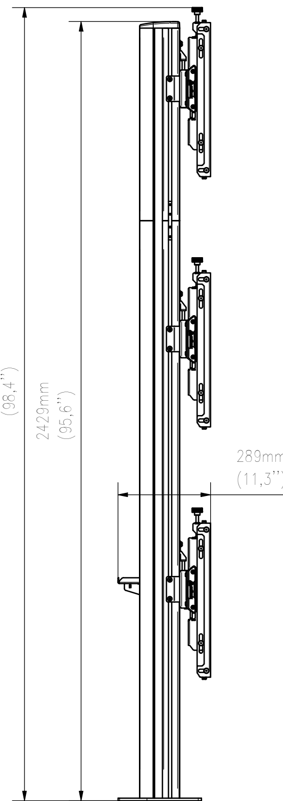
SIDE VIEW
